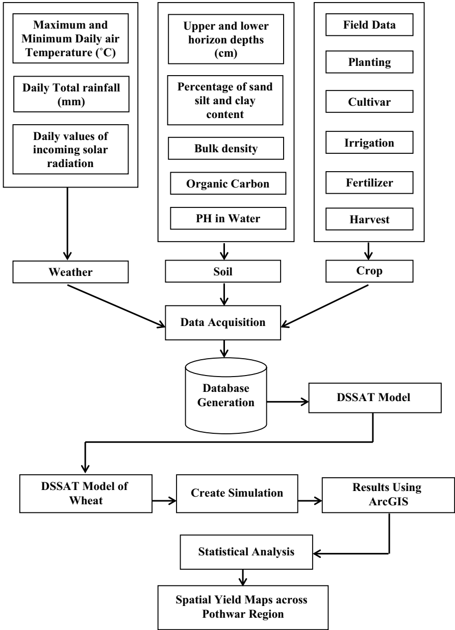
Fig. 16.2 Methodological framework
